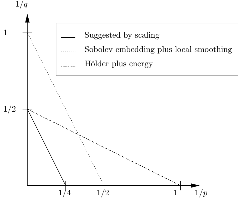
FIGURE 1. Fixed time scale, 1/2p derivative loss. The (p, q) relation suggested by scaling, from Sobolev embeddings plus local smoothing effect, and from Hölder's inequality in time with Sobolev embeddings and energy conservation.
